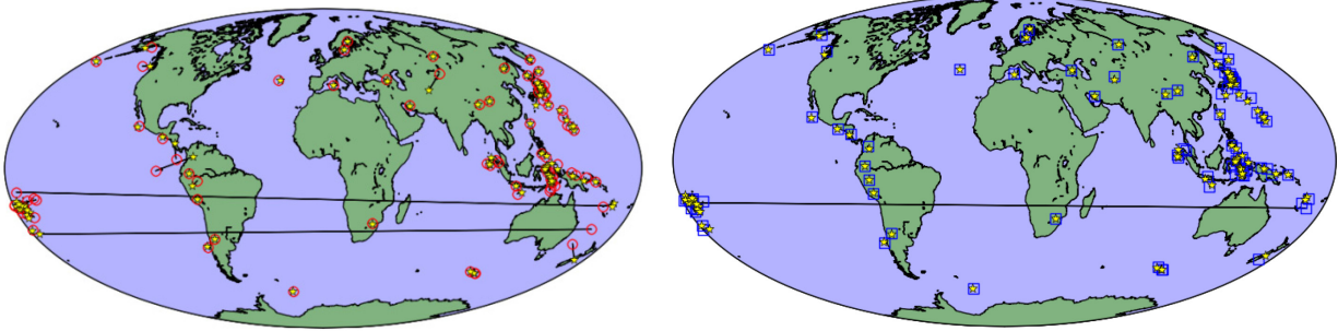
Figure 5. The changes in location of GA events (left figure, red circles) to the corresponding LEB events (yellow stars) and the changes in location of NET-VISA events (right figure, blue squares) to the corresponding LEB_VISA events (yellow stars). Straight lines (and not great circle lines) are drawn between corresponding events.
